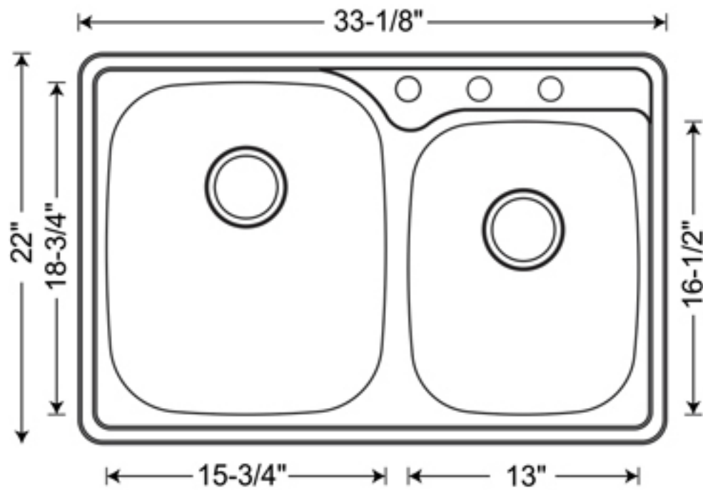
Depth = 9" & 7-1/2"
